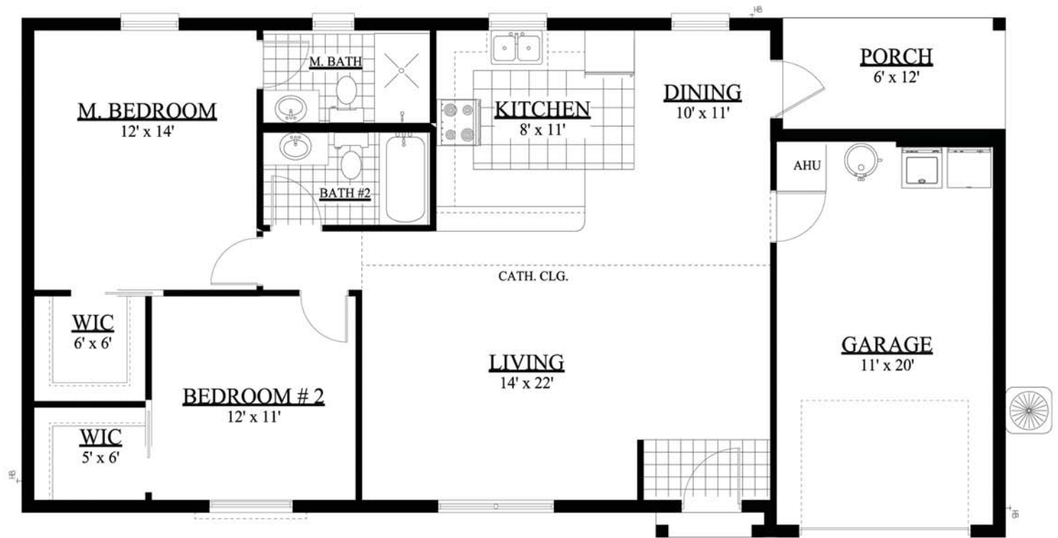
FLOOR PLAN
